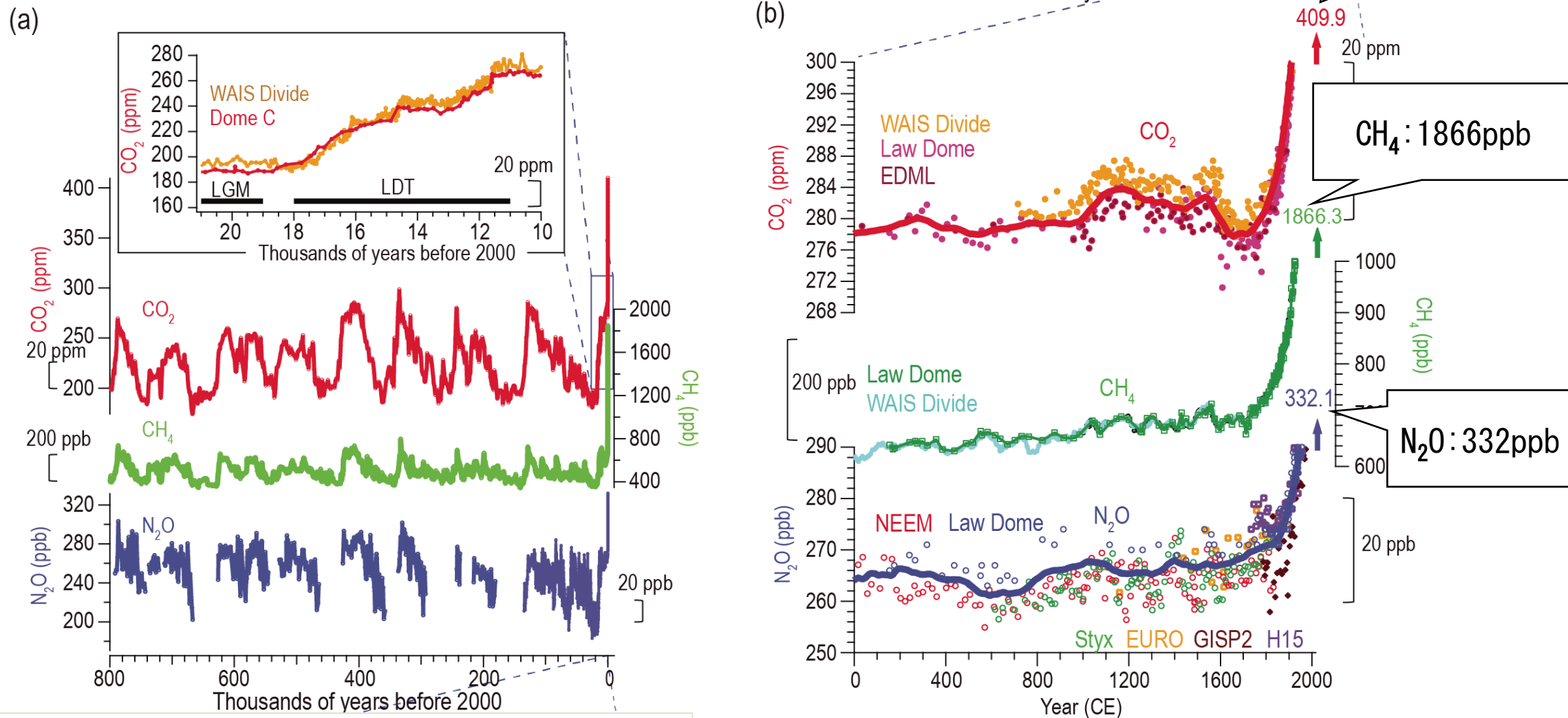
Evolution of well-mixed greenhouse gases
