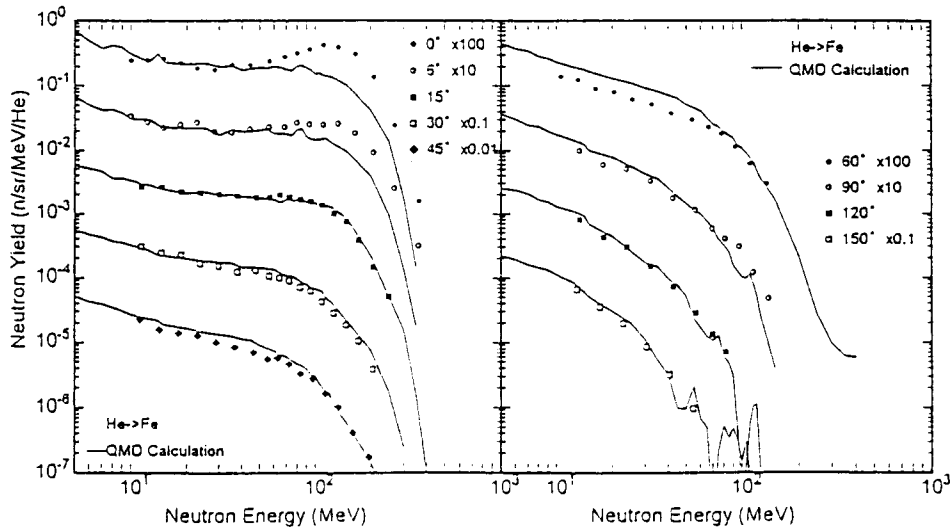
Fig. 2 Calculated double differential neutron yields of the iron target by QMD compared with the experimental data by 710 MeV alphas.
