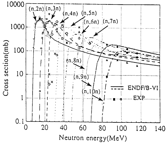
Fig. 1 Cross section data of ^{209}\text{Bi} (n,xn) reaction compared with ENDF/B-VI
